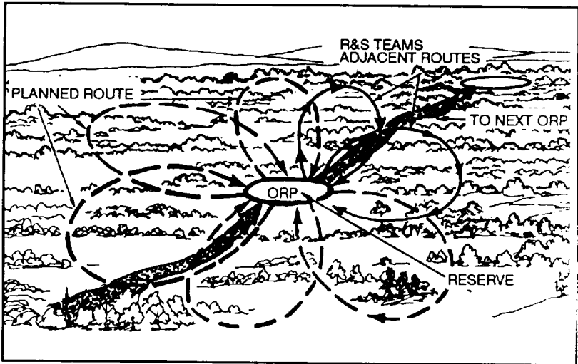
Figure 3-3. Fan method
